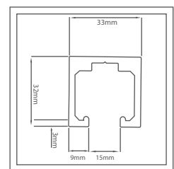
Top Track Dimension
